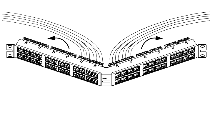
Recommended cable routing for terminated modules.
