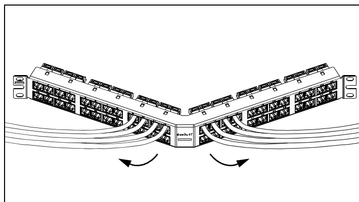
Recommended cable routing for patch cords.
